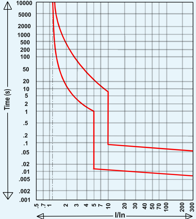
'C' Characteristics
